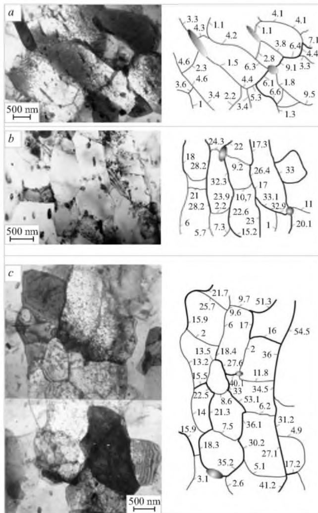
Fig. 1. Microstructures and grain-boundary maps (the numbers present the corresponding grain-boundary angles in degrees) of alloy 2219 deformed by ECAP at 250°C to a true degree of strain \varepsilon : a) \varepsilon = 2 ; b) \varepsilon = 4 ; c) \varepsilon = 8 .
