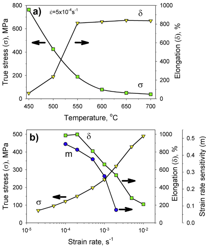
Fig. 12. Mechanical properties of ultrafine Ti–6Al–4V as a function of (a) deformation temperature at \dot{\epsilon} = 5 \times 10^{-4} \text{ s}^{-1} and (b) strain rate at T = 550 \text{ °C} . The stress level was defined at \epsilon = 0.2 .
