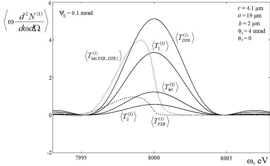
Fig. 7. Spectral-angular density of DTR \langle T_{DTR}^{(1)} \rangle , PXR \langle T_{PXR}^{(1)} \rangle and their interference term \langle T_{int}^{(1)}(PXR, DTR) \rangle . The other curves describe the terms forming the above-pointed term: T_{DTR}^{(s)} = T_1^{(s)} + T_2^{(s)} + T_{int}^{(s)} .
