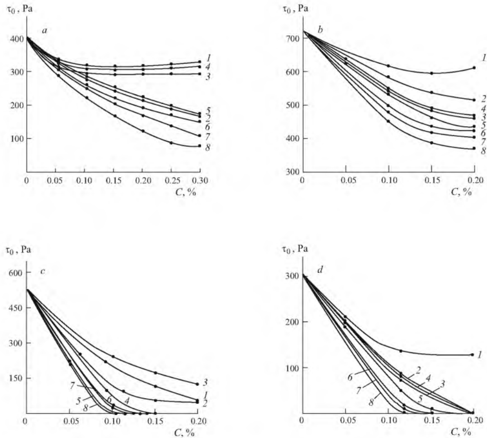
Fig. 1. Dependence of shear stress \tau_0 on the content C of additives in suspensions of clays VRC ( a ) and VSC ( b ), kaolin ( c ), and in ceramic slip ( d ): 1) water glass; 2) soda; 3) plasticizer S-3; 4) rheotan; 5) STPP; 6) rheotan + water glass + soda; 7) S-3 + water glass + soda; 8) S-3 + STPP.
