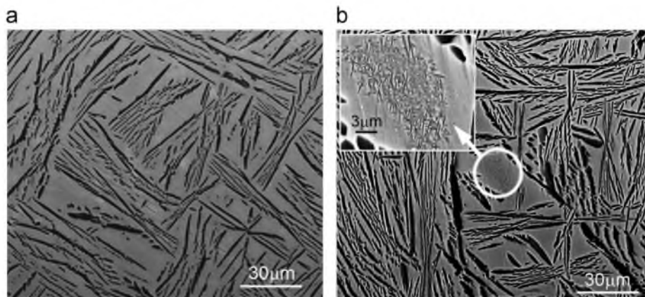
Fig. 2. SEM micrographs of the microstructure developed in Ti-5Al-5Mo-5V-1Cr-1Fe during preheating for 15 min (followed by water quenching) at (a) 800 °C or (b) 600 °C. The inset in (b) illustrates the decomposition of the \beta phase at higher magnification.
