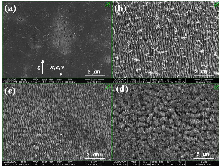
Figure 2. Low-magnification (10 000 \times ) SEM images of titanium surface nanostructured in air at N \approx 500 and F \approx 17 (a), 25 (b), 100 (c) и 250 (d) \text{mJ/cm}^2 .
