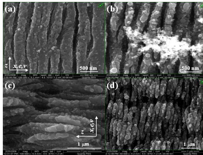
Figure 3. High-magnification SEM images of titanium surface nanostructured in air at N \approx 500 and F \approx 17 (a), 25 (b), 100 (c) и 250 (d) \text{mJ/cm}^2 at magnification of 100 000 \times (a-c) and 50 000 \times (d).
