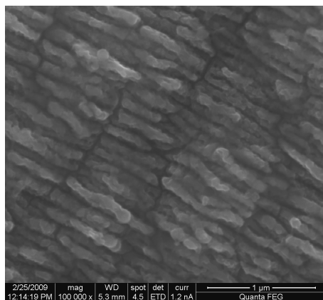
Figure 5. SEM image of the one-dimensional nanograting with the period \Lambda \approx 90 \text{ nm} written on the wet titanium surface at F \approx 300 \text{ mJ}/\text{cm}^2 and N \approx 500 .
