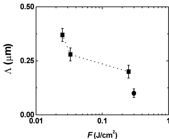
Figure 4. Periods \Lambda of one-dimensional nanogratings on dry (squares) and wet (circles) titanium surfaces versus F at N \approx 500 .
