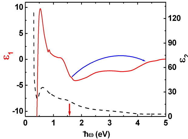
Figure 6. Optical spectra of real ( \varepsilon_1 , solid curve) and imaginary ( \varepsilon_2 , dashed curve) parts of dielectric function of titanium (after 18 ). The vertical arrow indicates the laser photon energy and the curved blue arrow shows the laser-induced spectral shift.
