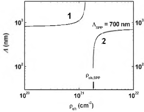
FIG. 5. Calculated SPP-wavelength \Lambda for the photoexcited graphite surface, vs \rho_{\text{eh}} . The branch 1 is unphysical [ \text{Re}(\varepsilon_1) + \text{Re}(\varepsilon_2) > 0 , \text{Re}(\varepsilon_1)\text{Re}(\varepsilon_2) > 0 ] compared to the branch 2 [ \text{Re}(\varepsilon_1) + \text{Re}(\varepsilon_2) < 0 , \text{Re}(\varepsilon_1)\text{Re}(\varepsilon_2) < 0 ]. The mark shows the SPP excitation threshold \rho_{\text{eh,SPP}} \approx 1.9 \times 10^{21} \text{ cm}^{-3} and the most probable SPP wavelength \Lambda_{\text{SPP}} \approx 700 \text{ nm} .
