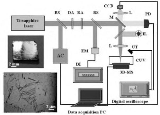
FIG. 1. Experimental setup for fs-laser surface nanostructuring: BS, beam splitter; AC, autocorrelator; DI, digital indicator; DA, RA, variable diffraction and reflective energy attenuators; EM, thermo-couple energy meter; M, mirror; L, focusing silica lenses; CCD, charge-coupled device camera for surface imaging; PD, fast trigger silicon photodiode; IL, illumination lamp; UT, ultrasonic transducer; CUV-plastic cuvette with the graphite sample for optional dry or wet nanostructuring; 3D-MS, three-dimensional motorized microstage. Insets: optical camera and microscope images of the HOPG piece.
