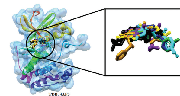
Figure 4. Enfolding of the 6 compounds in the active site pocket (1) ZINC00190959 Yellow, (2) ZINC07889110 Cyan, (3) ZINC00882851 Green, (4) ZINC01404326 Purple, (5) ZINC00882846 Blue, (6) ZINC08813187 Orange and VX-680 Black.
