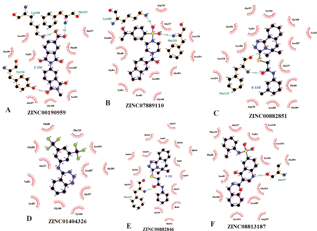
Figure 7. Ligplot+ results of schematic ligand interactions of the 6 candidates showing hydrogen-bond and hydrophobic interactions (A) ZINC00190959, (B) ZINC07889110, (C) ZINC00882851, (D) ZINC01404326, (E) ZINC00882846, (F) ZINC08813187.
