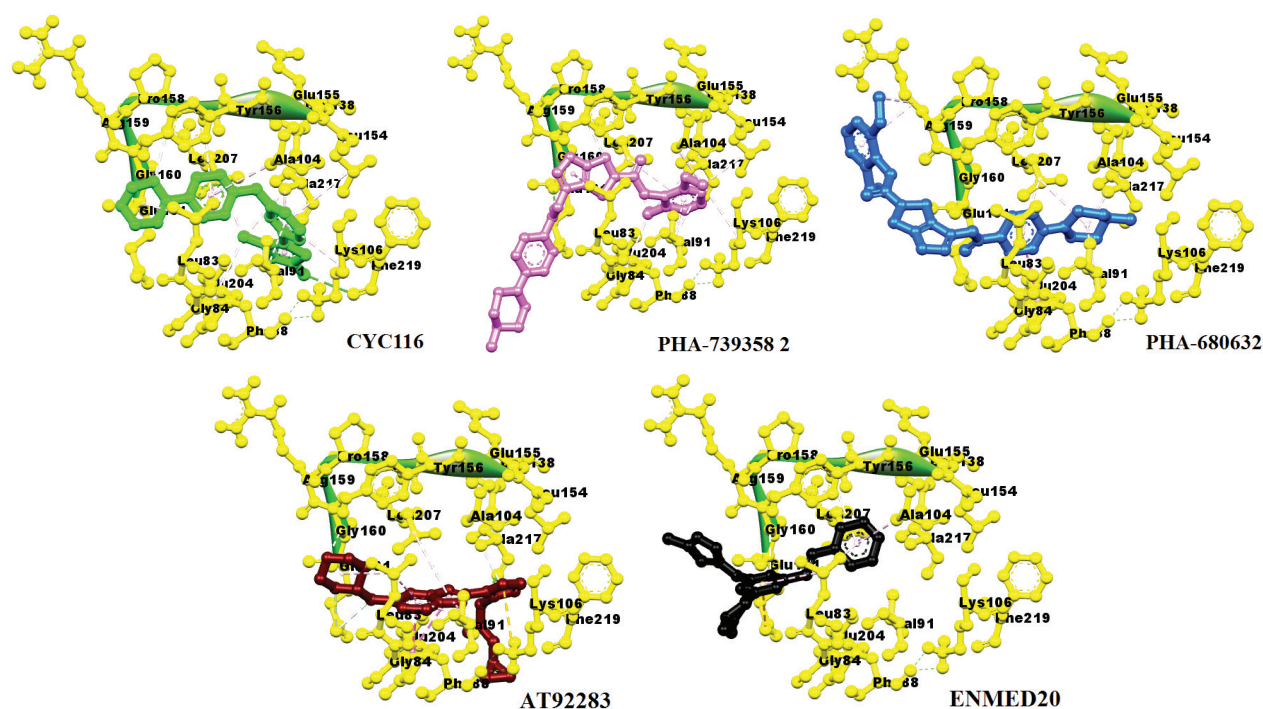
Figure 8. 3D structure of five clinical trial compounds used as Kinase AURK (A, B and C), namely CYC-116, PHA-739358, PHA-680632, AT9283 and ENMD-2076 in the binding pocket of (PDB:4AF3).
