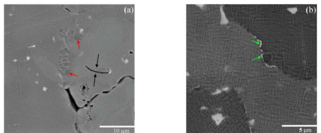
Figure 7. SEM-BSE images of the “large” specimen, upper half of the specimen. “Lack of fusion” defect is identified with black arrows. (a,b) Red and green arrows identify eutectic \gamma/\gamma' agglomerates and bulk or film-like carbides, respectively.
