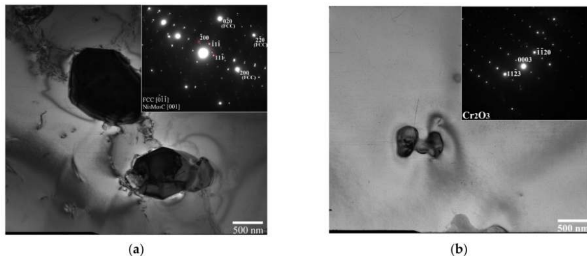
Figure 9. The microstructure of the “large” sample at level 1: particles of \text{Ni}_3\text{Mo}_3\text{C} phase (a), particles of \text{Cr}_2\text{O}_3 phase (b).
