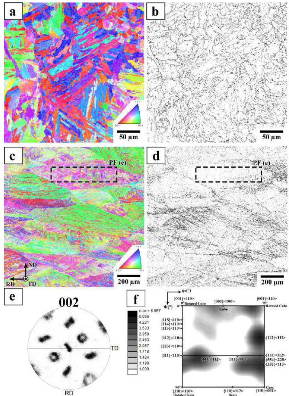
Figure 4. EBSD analysis of the untempered NT (a,b) and HR+Q (c–f) samples. Inverse pole figure maps for TD (a,c) and grain boundary maps showing the boundaries with misorientations between 20° and 49° to reveal PAGs (b,d). The <002> pole figure (e) and ODF ( \varphi_2 = 45^\circ section) of the HR+Q sample (f).
